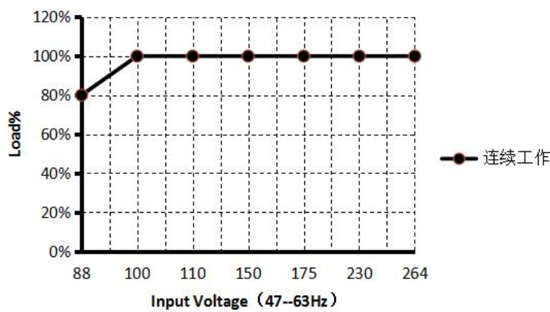
OUTPUT DERATING CURVE
