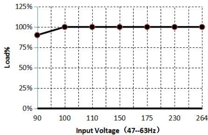
OUTPUT DERATING CURVE
