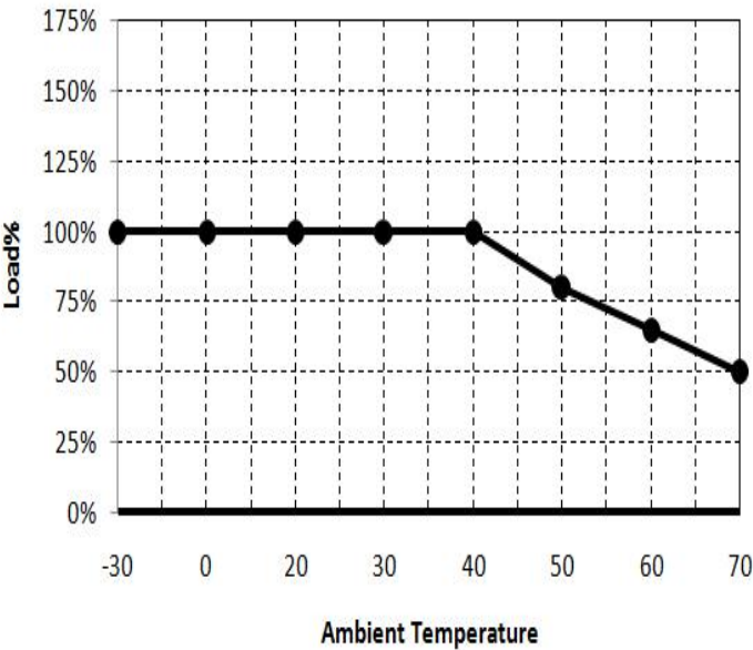
OUTPUT DERATING CURVE
